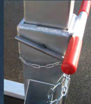
Optionally height-adjustable - good telescoping properties due to optimum tolerances
